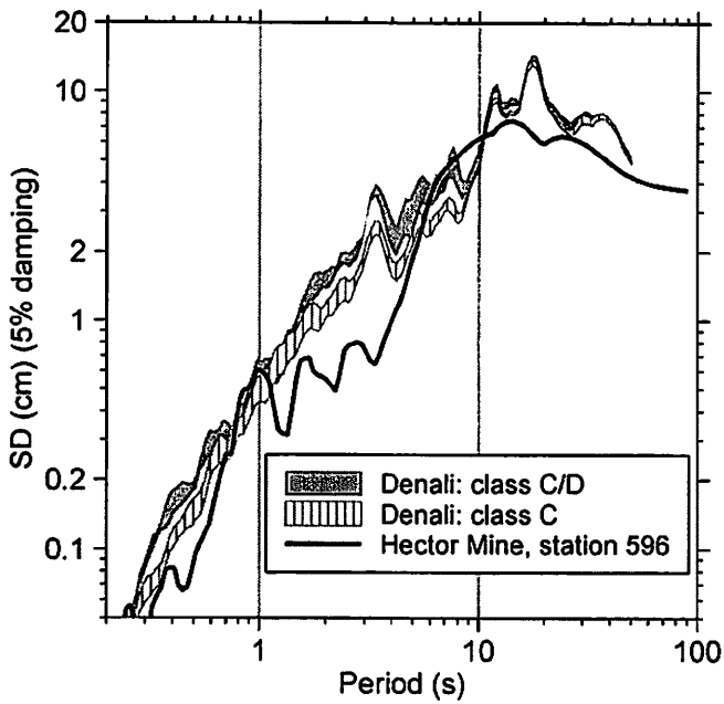
Figure 8. Displacement response spectrum (SD) for the 2002 Denali Fault, Alaska, earthquake recordings and for the transverse component of the 1999 Hector Mine, California, earthquake (after dividing the Hector Mine spectrum by 2.6 to correct for the different distances to the earthquakes). All records were low-cut filtered with a low-order acausal Butterworth filter with a corner at 0.02 Hz (the filter response goes as f^4 for low frequencies). (From Boore, 2004b).
