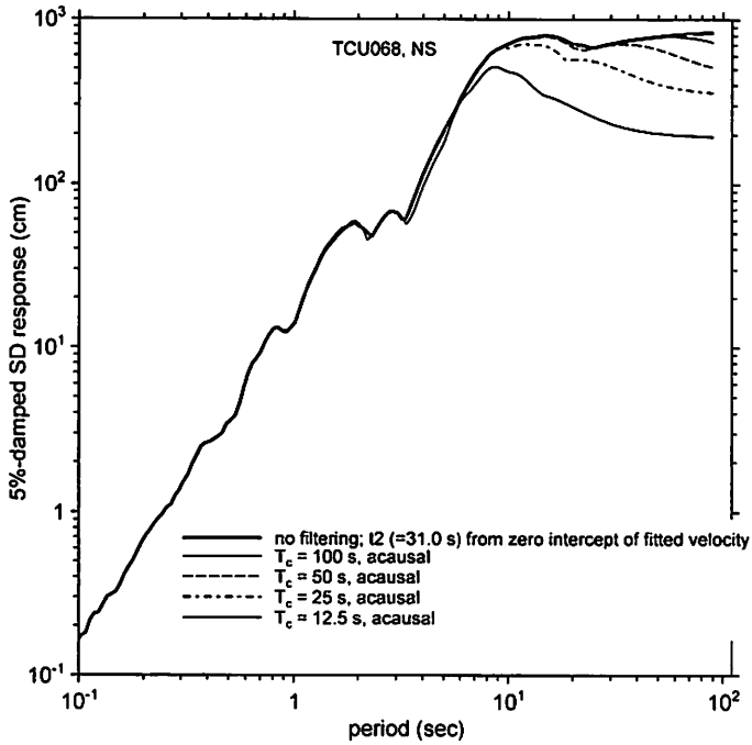
Figure 5. 5%-damped relative displacement response spectra for the time series processed using acausal filters.
