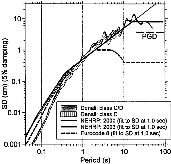
Figure 10. Comparison of observed displacement response spectrum (SD) for class C/D and C sites in Anchorage to the spectra constructed following the procedures for the following building codes: 2000 NEHRP (BSSC, 2001), 2003 NEHRP (BSSC, 2004), and Eurocode 8 (CEN, 1998). Also shown is the peak ground displacement (PGD) for the Anchorage motions; the displacement response spectrum will be asymptotic to this value at sufficiently long periods. For NEHRP, the mapped values of spectral response at 0.2 and 1.0 s were used, but to emphasize the shape, the spectra for the three codes have been normalized to a representative value of the data at 1 s. (From Boore, 2004b.)
