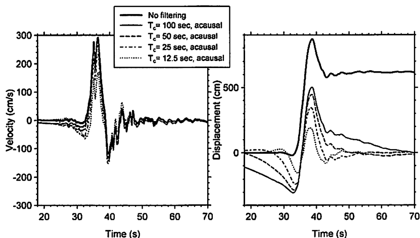
Figure 4. The velocity and displacement time series derived from the TCU068 recording. In all cases a simple baseline correction (the “v0” correction of Boore, 2001) was used, with and without filtering. The filters were low-cut acausal Butterworth filters having filter corner periods of 12.5, 25, 50, and 100 sec.
