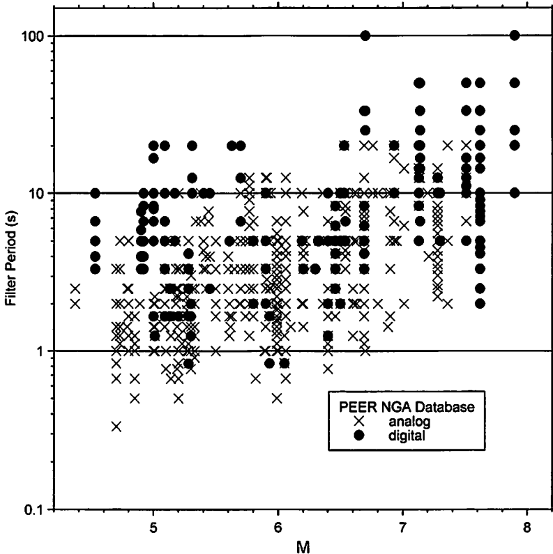
Figure 6. Filter period vs. moment magnitude, with data from analog and digital instruments indicated by the symbols. An effort has been made to determine whether each recording was made on an analog or a digital instrument, but there are undoubtedly a few errors. The filter for which the period is given removes long-period energy from the record, and the filter periods are those in a database being developed for use in the Pacific Earthquake Engineering Research Center (PEER) New Generation Attenuation (NGA) project. An attempt has been made in developing the PEER NGA database to apply uniform processing to all records. Some of the recordings, such as the analog recordings of the M 7.4 Tabas, Iran earthquake, may have had significant amounts of long-period noise removed by the use of baseline corrections, in which case the filter period is not a good measure of the long-period content of the record. For this reason the Tabas data are not shown here. In some other cases, such as the M 7.6 1999 Chi-Chi, Taiwan earthquake, longer filter periods could have been chosen.
