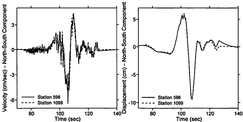
Figure 7. Comparison of a) velocities and b) displacements for two closely spaced (1.6 km) stations that recorded the 1999 Hector Mine, California, earthquake. The recorded accelerations from which the velocities and displacements are derived were processed using a constrained quadratic fit to velocity, followed by acausal filtering with a corner frequency of 0.02 Hz. The traces are aligned using time shifts derived by visually aligning the large pulse to the south on the displacement trace. (From Boore et al., 2002, but using acausal rather than causal filtering.)
