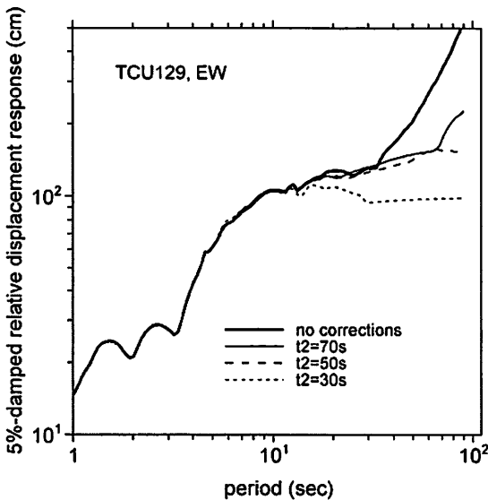
Figure 3. Displacement response spectra corresponding to processing shown in the previous figure.
