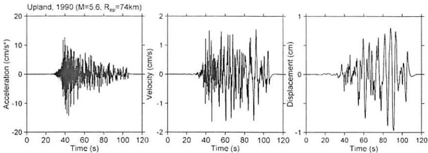
Figure 1. Acceleration, velocity, and displacement time series for one horizontal component of a 16-bit recording of the 1990 Upland earthquake, with a 0.1 Hz acausal low-cut filter. The waves traveling to the station have traversed part of the Los Angeles basin, and therefore large surface waves are present on the displacement time series. (From Boore, 2004a.)
