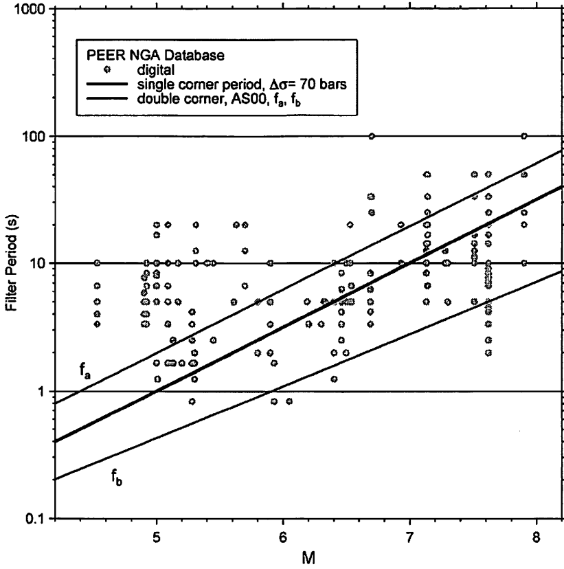
Figure 9. Corner periods from two source-scaling models, compared to the filter periods used in processing strong-motion data (AS00 = Atkinson and Silva, 2000).
