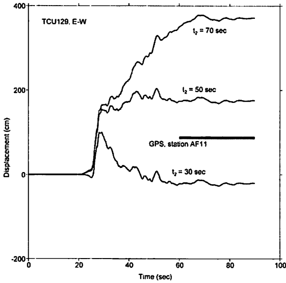
Figure 2. Displacements obtained by double integration of the EW component of acceleration recorded at TCU129 and modified using three values of T_2 to correct for baseline shifts. The GPS level was obtained at a station 2.3 km from TCU129, on the foot wall side of the fault (as is TCU129). (Modified from Boore, 2001.)
