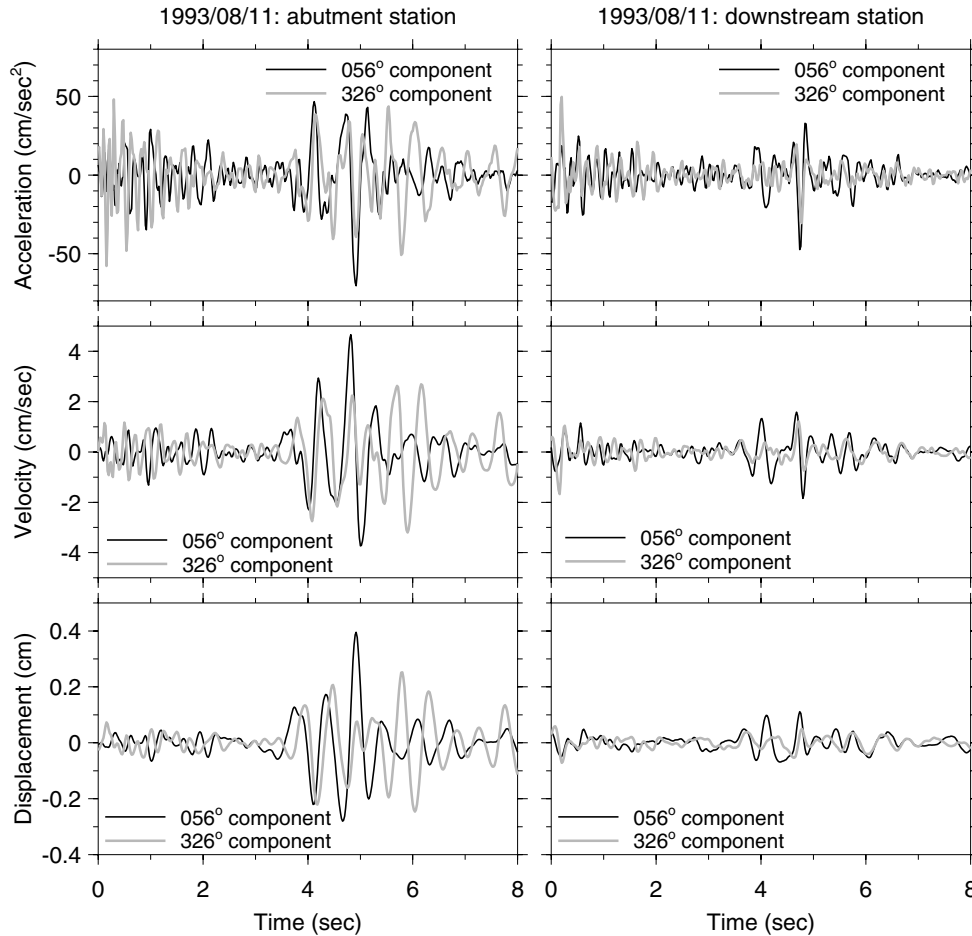
Figure 8. Acceleration, velocity, and displacement time series from the 11 August 1993 earthquake, recorded at the abutment and downstream stations. Shown is the horizontal motion rotated into a direction normal ( 56^\circ ) and parallel ( 326^\circ ) to the fault strike. Absolute time was not available for the record.
