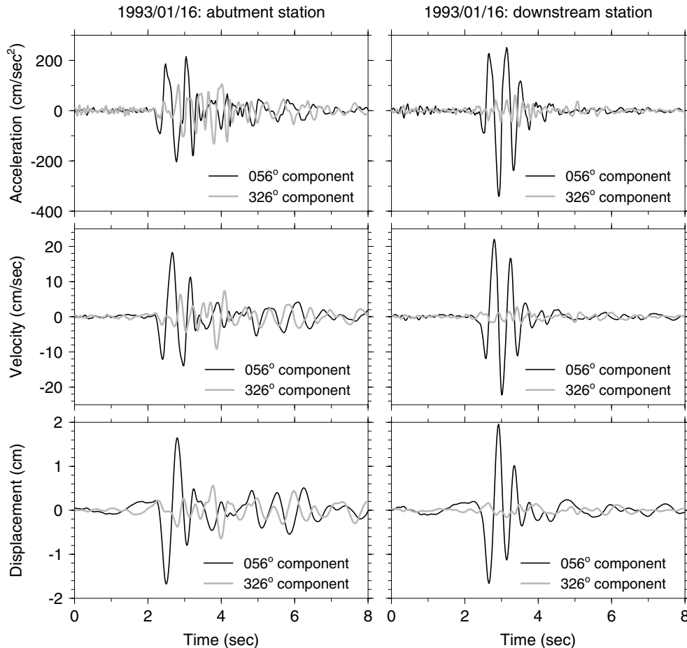
Figure 7. Acceleration, velocity, and displacement time series from the 16 January 1993 earthquake, recorded at the abutment and downstream stations. Shown is the horizontal motion rotated into a direction normal ( 56^\circ ) and parallel ( 326^\circ ) to the fault strike. Absolute time was not available for the record. The polarization for this event is dominated by fault-normal motion, unlike the motion from earlier events, and the motion is generally larger on the downstream site than on the abutment site, again unlike the previously shown events.
