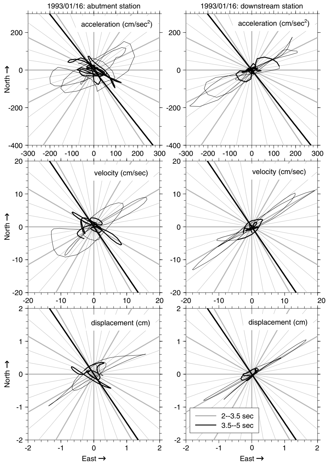
Figure 11. Hodograms of the horizontal components of motion for the 16 January 1993 earthquake, at the abutment and the downstream sites. Plot labeling as in Figure 9, except the records are for recordings of same earthquake (16 January 1993) at the two stations. The thin and thick lines indicate time segments of 2.0–3.5 and 3.5–5.0 sec, respectively. The first window was chosen so as to contain the maximum accelerations (see Fig. 7). The accelerograms for both stations and both components were low-cut and high-cut filtered using ramps between 0.3 and 0.6 Hz and between 23 and 25 Hz, respectively.
