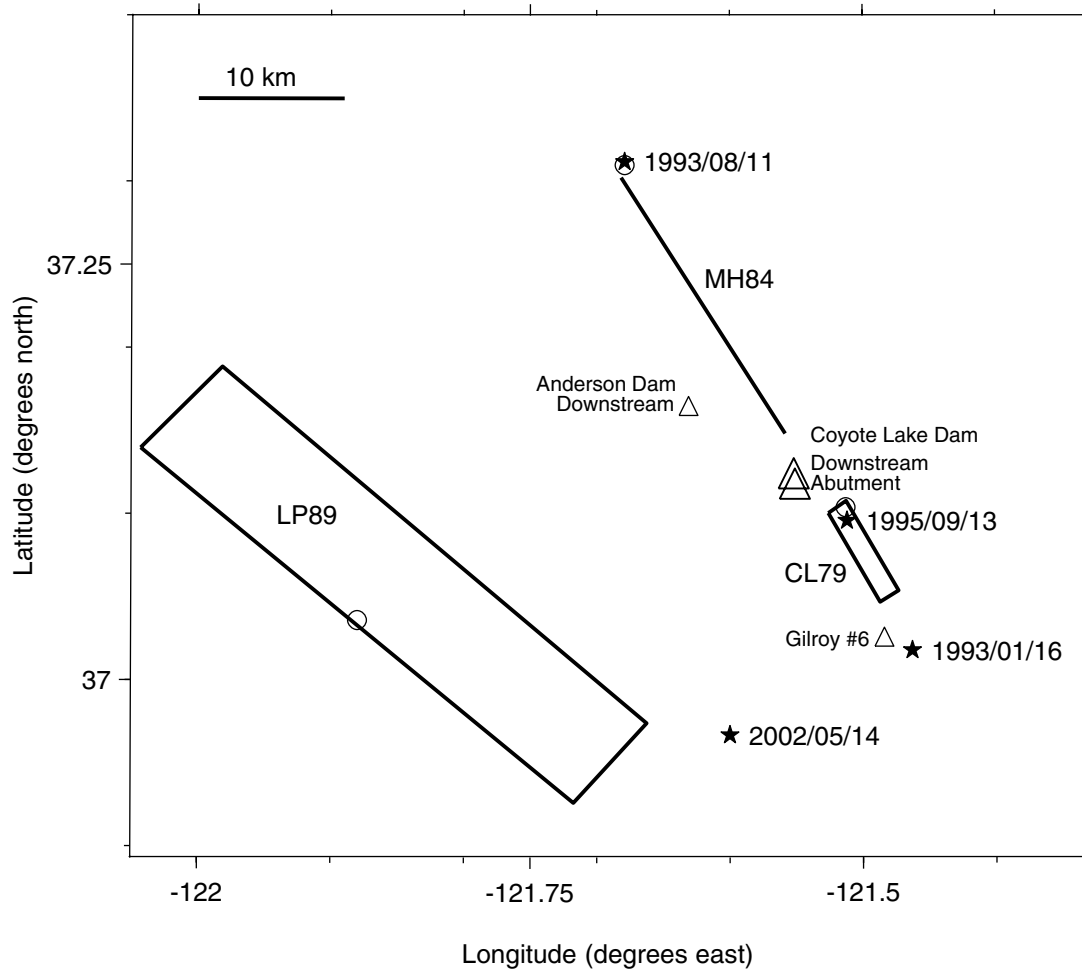
Figure 1. Location of the earthquakes recorded at the Coyote Lake Dam stations. The Coyote Lake Dam stations are shown by large triangles; the small triangles are other stations discussed in the article. The surface projection of a rectangle approximating the rupture surface (after Spudich and Olsen, 2001) is shown for the 1979 Coyote Lake (CL79 = 6 August 1979), 1984 Morgan Hill (MH84 = 24 April 1984), and 1989 Loma Prieta (LP89 = 18 October 1989) earthquakes; the epicenters for these three events are shown by open circles. The epicenters of the other events are shown by stars. All events were recorded at the abutment station, and all but the 1979 and 1984 events were recorded at the downstream station. The events 13 September 1995 and 14 May 2002 produced records too small to be digitized; only the peak accelerations for those events are used in this article.
