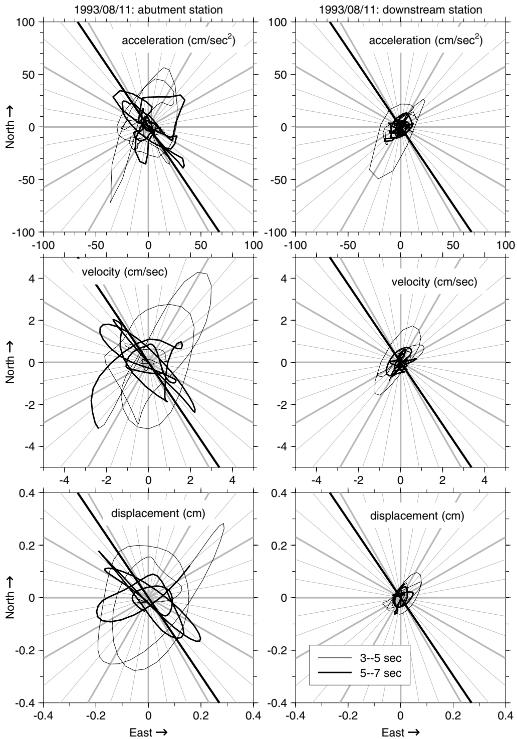
Figure 12. Hodograms of the horizontal components of motion for the 11 August 1993 earthquake, at the abutment and the downstream sites. Plot labeling is as in Figure 9, except the records are for recordings of the same earthquake (11 August 1993) at the two stations. The thin and thick lines indicate time segments of 3.0–5.0 and 5.0–7.0 sec, respectively. The first window was chosen so as to contain the maximum accelerations (see Fig. 8). The accelerograms for both stations and both components were low-cut and high-cut filtered using ramps between 0.4 and 0.8 Hz and between 23 and 25 Hz, respectively.
