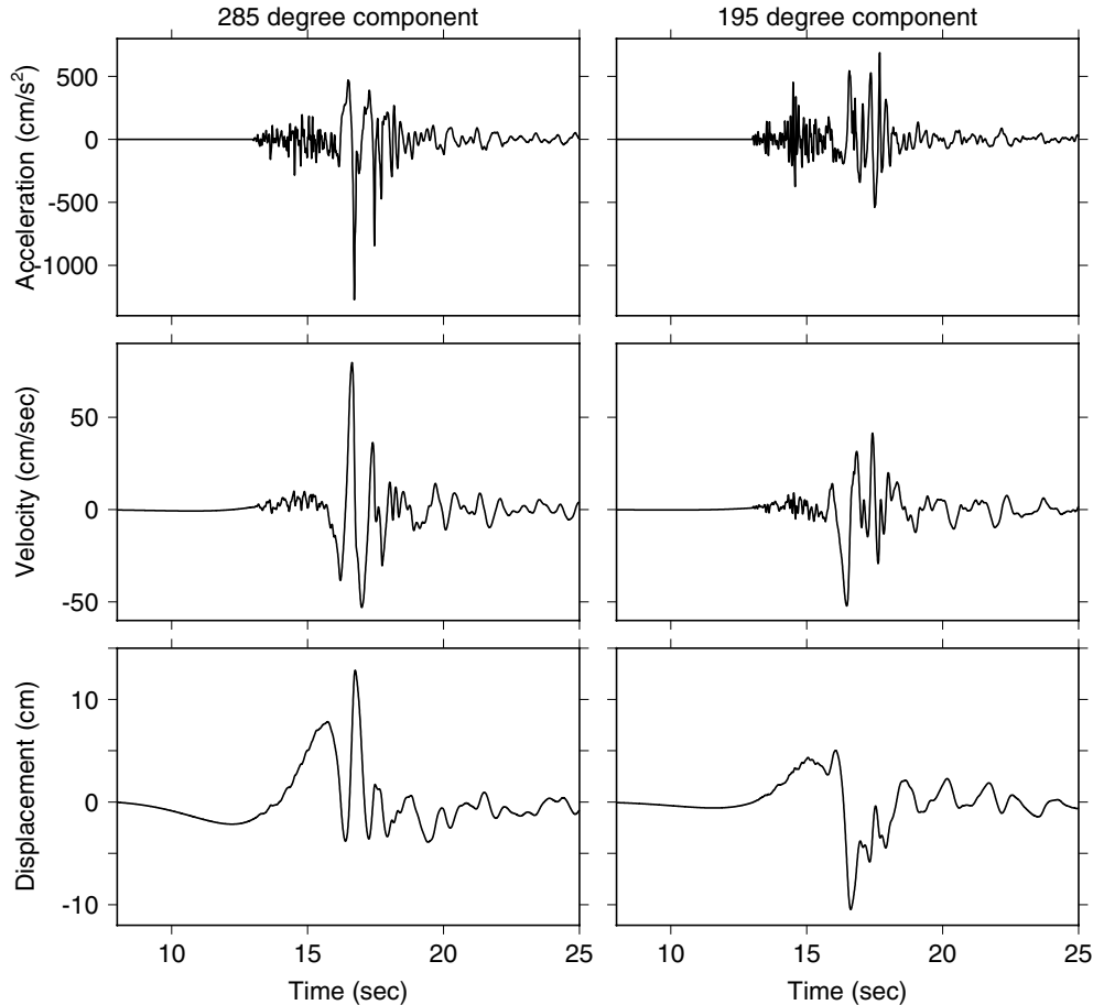
Figure 2. Acceleration, velocity, and displacement time series for the two horizontal components of motion from the 1984 Morgan Hill earthquake, recorded at the Coyote Lake abutment station. Note the large pulse of acceleration on the 285° component. The component directions are in degrees clockwise from north. The acceleration traces are unfiltered; the velocity and displacement traces were obtained by integration of filtered acceleration traces. The acceleration traces for both components were padded with 13 sec of zeros before and after the motion and were filtered using a zero-phase Butterworth low-cut filter with corner frequency of 0.12 Hz. The order of the filter was chosen so that its response goes as f^4 for low frequencies. The large pre-S motion in the displacement traces is a consequence of the interaction of the acausal filter response and the large peak in acceleration; it cannot be reduced by tapering of the motions near the start of the record. The only way of reducing its effect is to choose a higher low-cut frequency.
