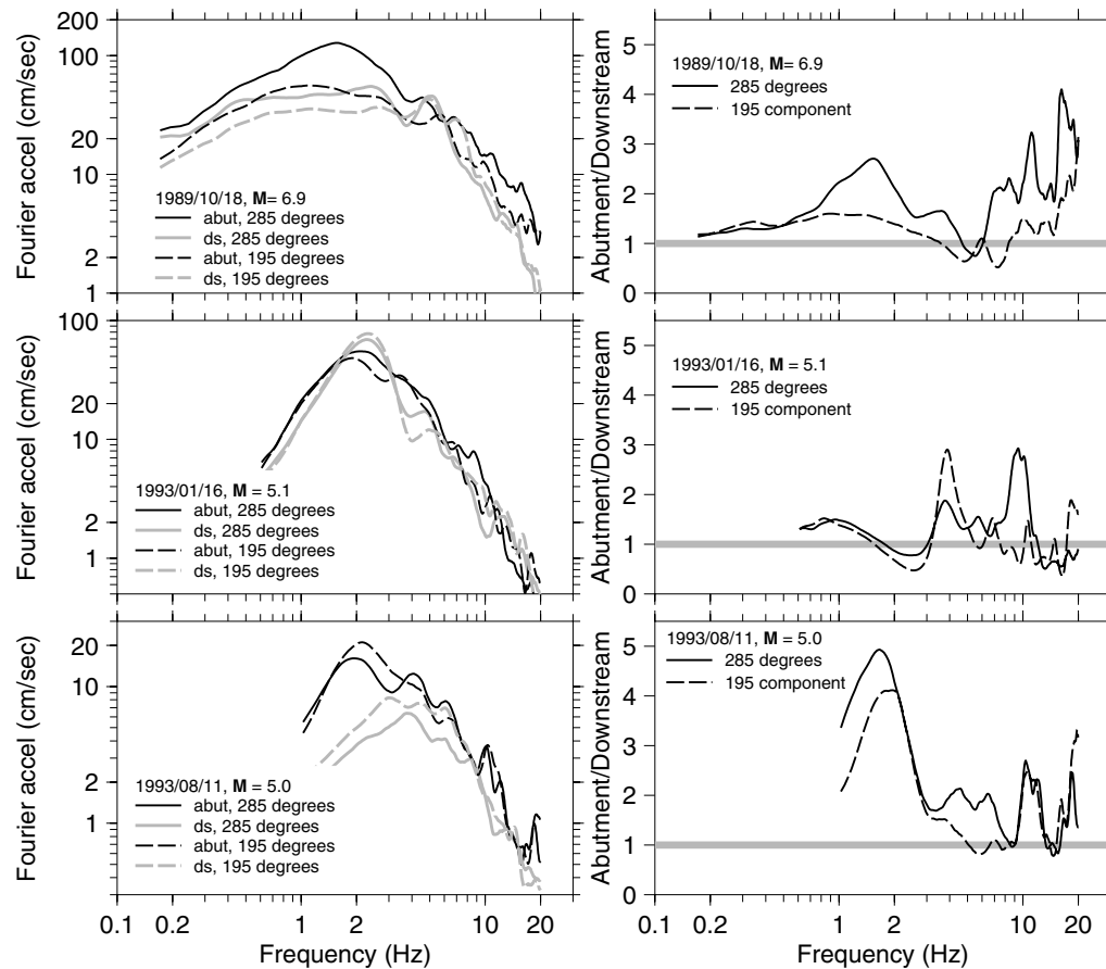
Figure 13. Fourier spectra (left column of graphs) and spectral ratios (right column of graphs) of the three events recorded at both the abutment and downstream stations for which the analog records were large enough to be digitized. The spectra for the frequency range shown are judged to be well above the noise. The spectra of the two stations have been smoothed using a triangular smoothing function with half-width of 1 Hz before forming the ratio. The Fourier spectra are plotted using logarithmic scaling for the ordinate to allow the reader to judge the spectral ratios shown in the right column of graphs.
