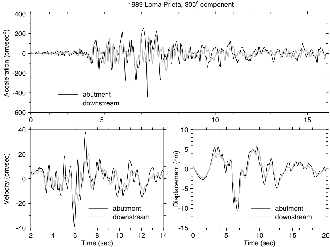
Figure 6. Acceleration, velocity, and displacement time series from the 1989 Loma Prieta earthquake, recorded at the abutment and downstream stations. The traces have been aligned to start at the same absolute time (00:04:24.6 UTC). Shown is the horizontal motion rotated into a direction corresponding to the peak polarization determined from the velocity traces. Note that the time-axis scaling is different for the acceleration, velocity, and displacement traces. This was done to make it easier to compare the abutment and downstream motions. For the displacements, the motions at the two stations are very similar, but at higher frequencies (as shown in the velocity and acceleration traces) the correlation starts to break down after the first arrival, and the abutment station motion is generally larger than the downstream station motion.
