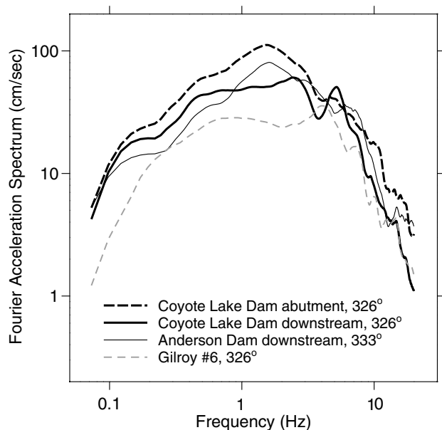
Figure 14. Fourier acceleration spectra for four recordings of the 1989 Loma Prieta earthquake at somewhat comparable distances from the surface projection of the fault rupture: Anderson Dam downstream (18.0 km), Coyote Lake Dam downstream (19.0 km), Gilroy 6 (17.0 km), and, for comparison, Coyote Lake Dam abutment (18.5 km) (see Fig. 1 for station locations). Corrections for geometric spreading were not applied; they are less than a factor of 0.92 (the factor to go from Gilroy 6 to Coyote Lake downstream). Except for Anderson Dam downstream, the spectra are shown for the fault-parallel component; for Anderson Dam downstream particle motion plots show elliptical polarization, which is probably due to the two traces not being precisely aligned in time when digitized. Fortunately, the as-recorded component of 333^\circ is close to the fault-parallel direction. Both Gilroy 6 and Coyote Lake Dam downstream are slightly to the east of the Calaveras fault zone; Anderson Dam downstream is to the west of the fault zone. Both the Anderson Dam and the Gilroy 6 sites fall into National Earthquake Hazard Reduction Program (NEHRP) class C, with average shear-wave velocities to 30 m of 489 and 589 m/sec, respectively. The velocities at the Coyote Lake Dam sites have not been measured, but it is likely that the sites would fall into the NEHRP class C category ( 360 \text{ m/sec} < \bar{V}_s[30 \text{ m}] \leq 760 \text{ m/sec} ).
