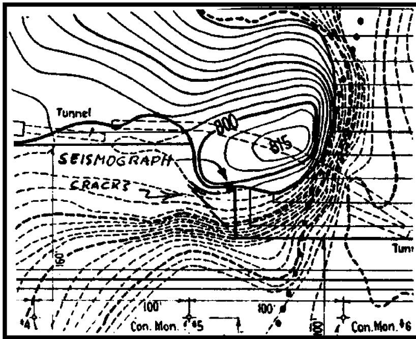
Figure 5. As-constructed drawing from Tepel (1984), showing predam (dashed where under present-day topography) and postdam (solid) contours (contour interval is 5 ft). The parallel set of contours show the upstream and downstream faces of the dam. The downstream face slopes toward the top of the figure.
